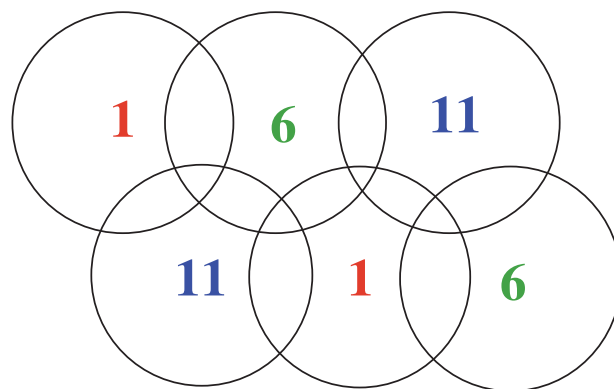
Figure 3 Channel assignment causing no interference
