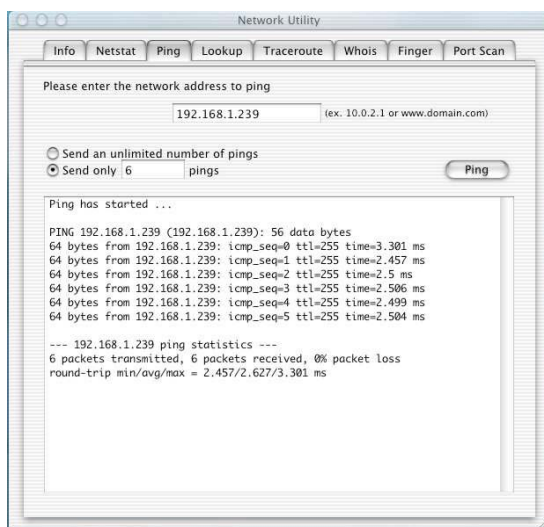
Figure 2 Unix command Ping
